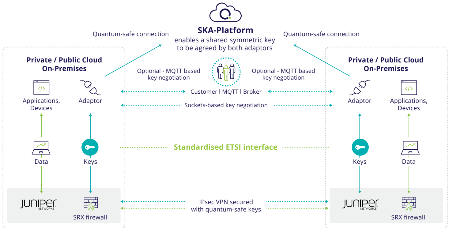
Figure 1. Arqit NetworkSecure Adaptor integration with SRX to deliver quantum-secure symmetric keys via ETSI 014 interface
