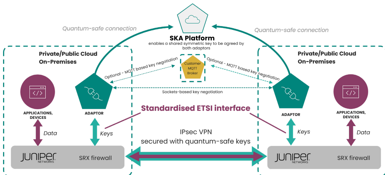
Figure 1. Arqit NetworkSecure Adaptor integration with SRX to deliver quantum-secure symmetric keys via ETSI 014 interface
