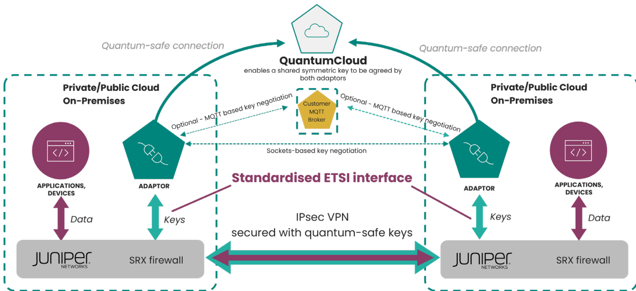
Figure 1. Arqit QuantumCloud NetworkSecure Adaptor integration with SRX to deliver quantum secure symmetric keys via ETSI 014 interface
