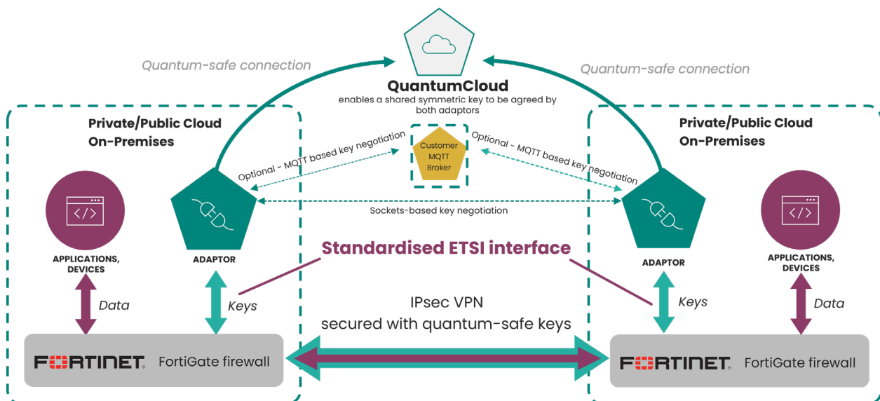
Figure 1. Arqit QuantumCloud NetworkSecure Adaptor integration with FortiGate to deliver quantum secure symmetric keys via ETSI 014 interface
